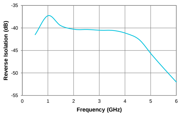
Reverse Isolation
