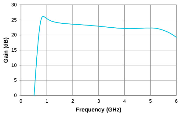
Insertion Gain
