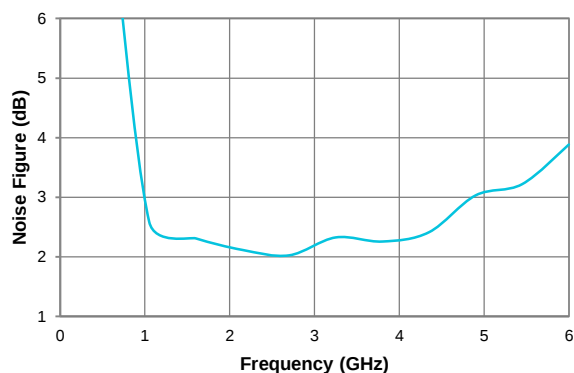
Noise Figure
