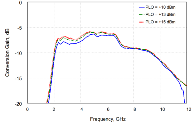
Conversion Gain vs. LO Drive @IF = 2 GHz
