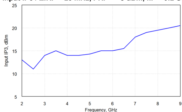
Input IP3 / \Delta f_{RF} = 10 MHz, PRF = -5 dBm, fIF = 0.1 GHz
