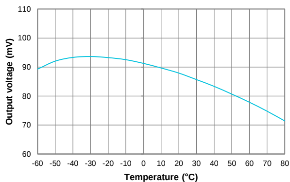
Vdet vs. Temp., f = 1 GHz, P IN = 10 dBm
