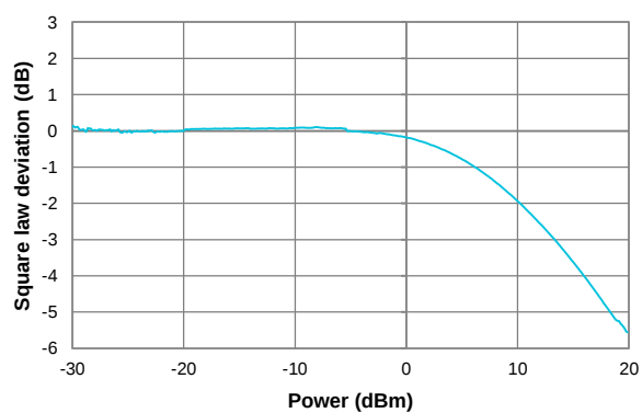
Square law deviation
